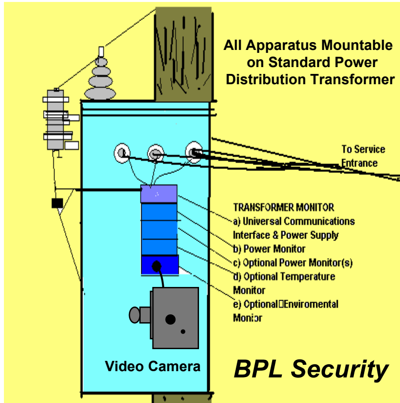
BPL Surveillance & Security System
